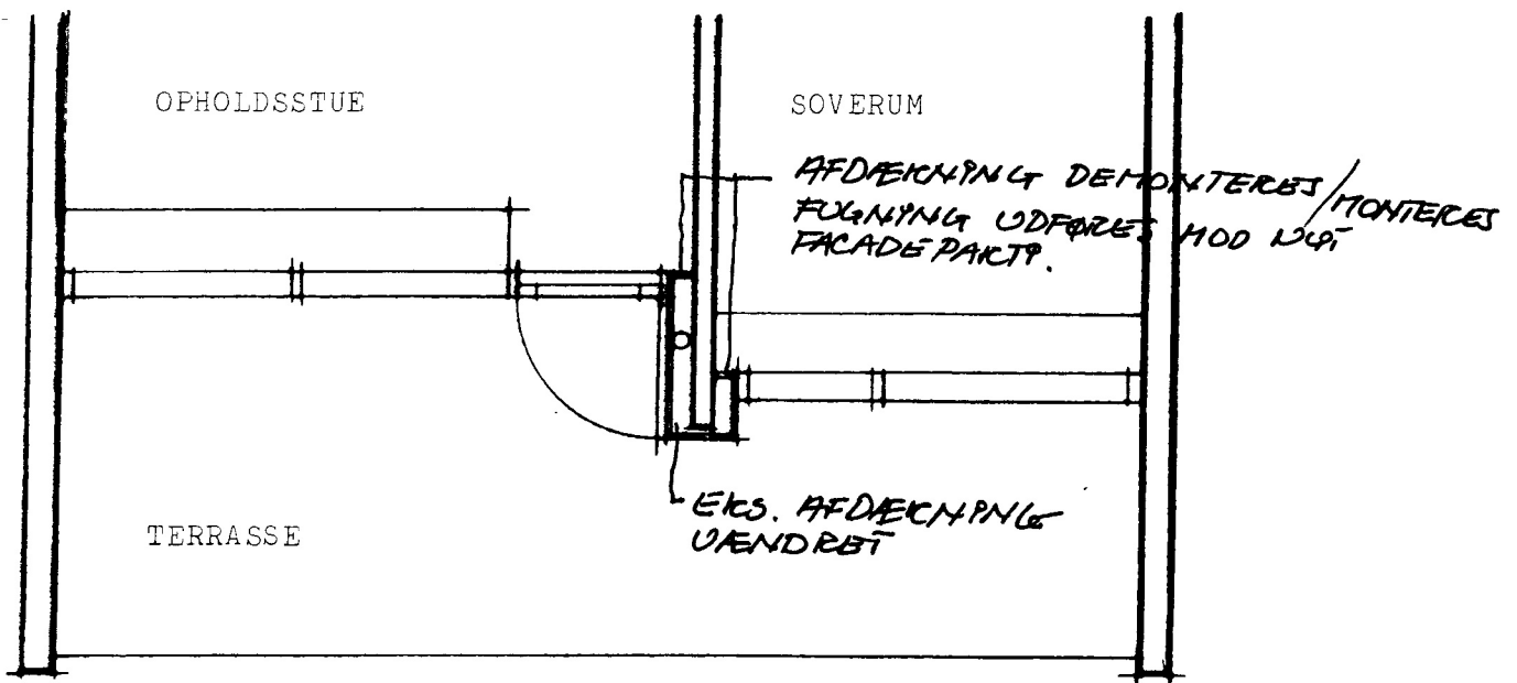
Plan - facadeparti 1:50
