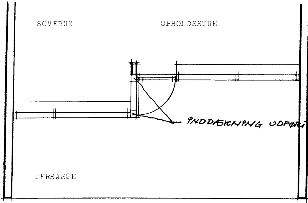
Plan - facadeparti 1:50
